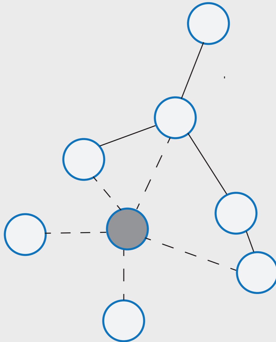
Figure 8.3 Software complexity
